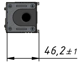
Mounting bracket Set 19" 1HU M03.551-3F
